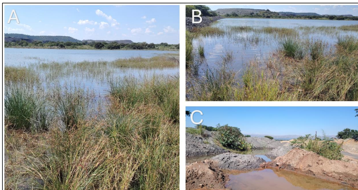
Figure 4-8 Diagnostic soil horizons identified on-site: A-C) Examples of surface return/overland flows and lateral flows pathways
