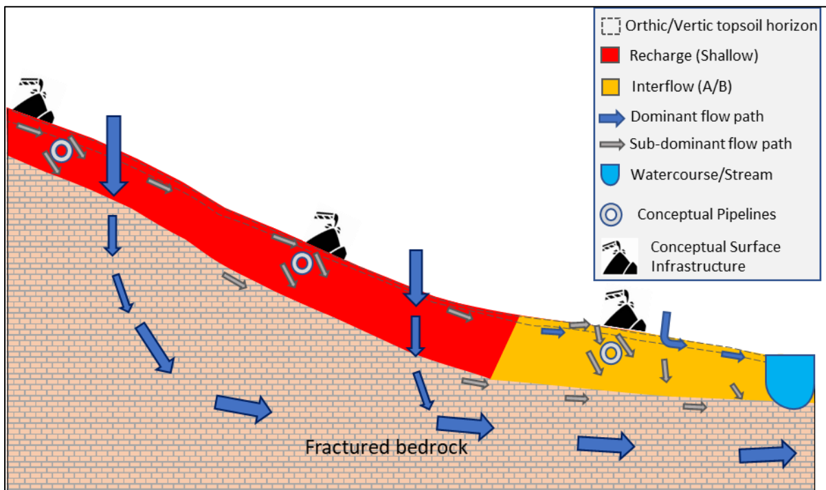
Figure 4-16 Hillslope hydrology three of five of the distinct hydropedological patterns after the construction of the Clover Alloys SA Plant Infrastructure Project and associated infrastructure
