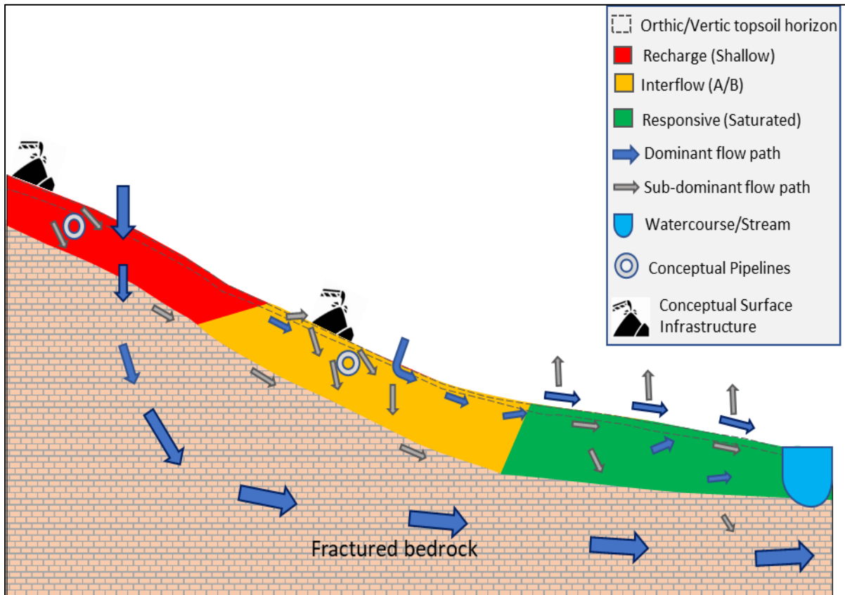
Figure 4-18 Hillslope hydrology five of five of the distinct hydro-pedological patterns after the construction of the Clover Alloys SA Plant Infrastructure Project and associated infrastructure
