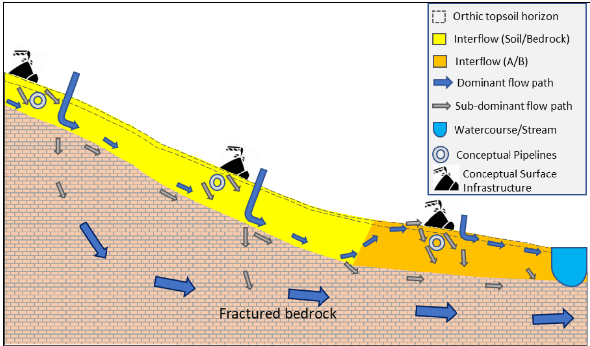
Figure 4-17 Hillslope hydrology four of five of the distinct hydro-pedological patterns after the construction of the Clover Alloys SA Plant Infrastructure Project and associated infrastructure
