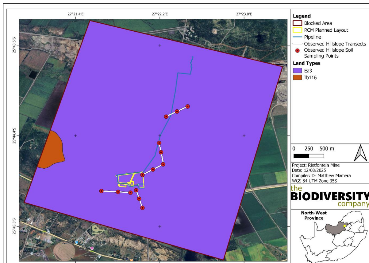
Figure 4-4 Land types present within the Clover Alloys SA Plant Project's surroundings
