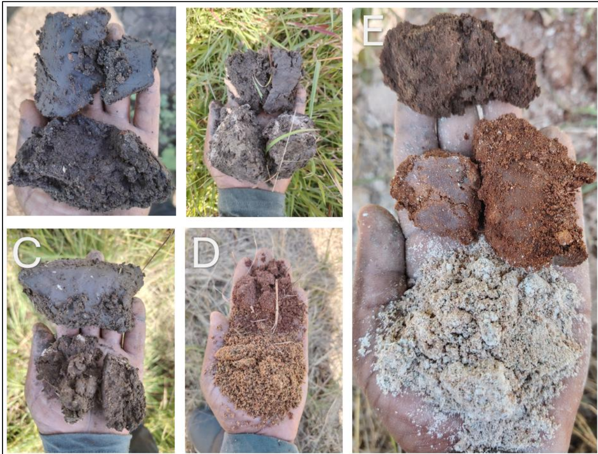
Figure 4-6 Diagnostic soil horizons identified on-site: A-C) Vertic horizons. D) Transported material. D) Orthic topsoil horizon with a lithic horizon. E) Neocutanic subsurface horizon with soft carbonate
