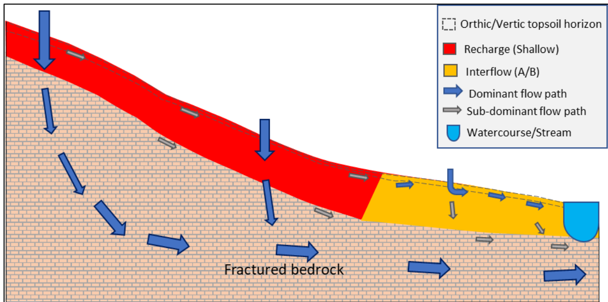
Figure 4-11 Hillslope hydrology three of five of the distinct hydropedological patterns prior to construction of the Clover Alloys SA Plant Infrastructure Project and associated infrastructure.
