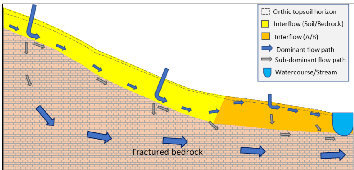
Figure 4-12 Hillslope hydrology four of five of the distinct hydropedological patterns prior to construction of the Clover Alloys SA Plant Infrastructure Project and associated infrastructure.
