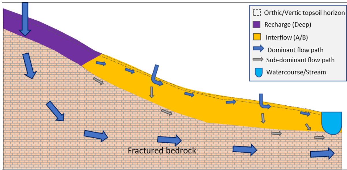
Figure 4-9 Hillslope hydrology one of five of the distinct hydropedological patterns prior to construction of the Clover Alloys SA Plant Infrastructure Project and associated infrastructure.
