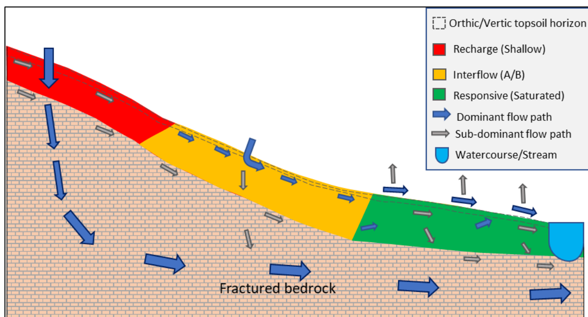
Figure 4-13 Hillslope hydrology four of five of the distinct hydropedological patterns prior to construction of the Clover Alloys SA Plant Infrastructure Project and associated infrastructure.
