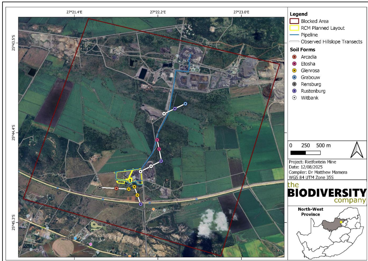
Figure 4-5 Soil forms identified within representative hillslope transects
