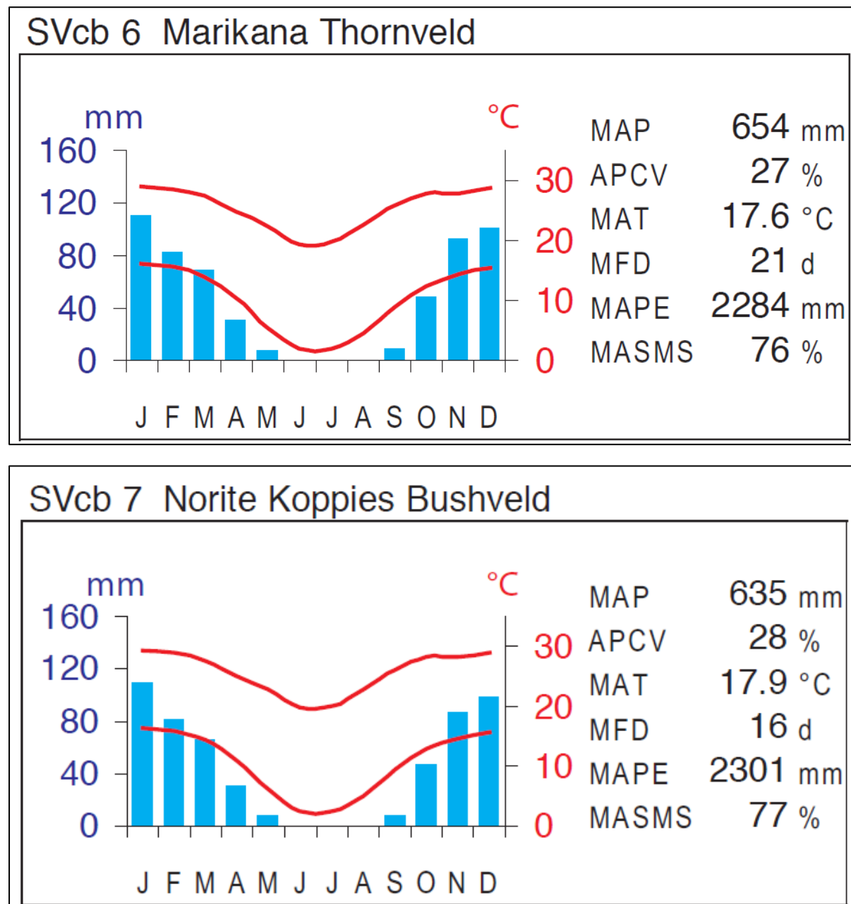
Figure 4-1 Summarised climate for the region (Mucina & Rutherford, 2006)
