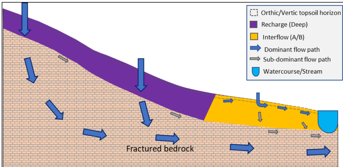
Figure 4-10 Hillslope hydrology two of five of the distinct hydropedological patterns prior to construction of the Clover Alloys SA Plant Infrastructure Project and associated infrastructure.
