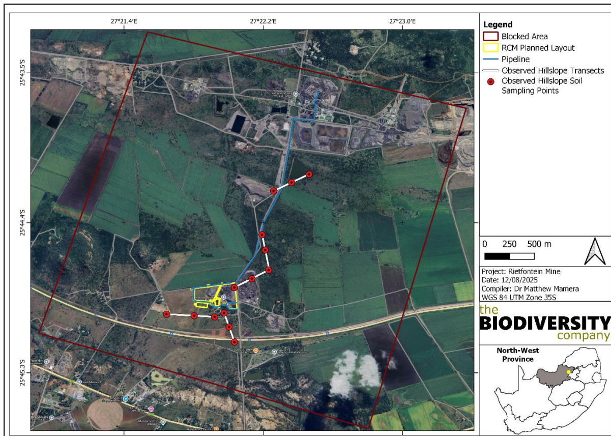
Figure 3-1 Transects and Observation Sites
