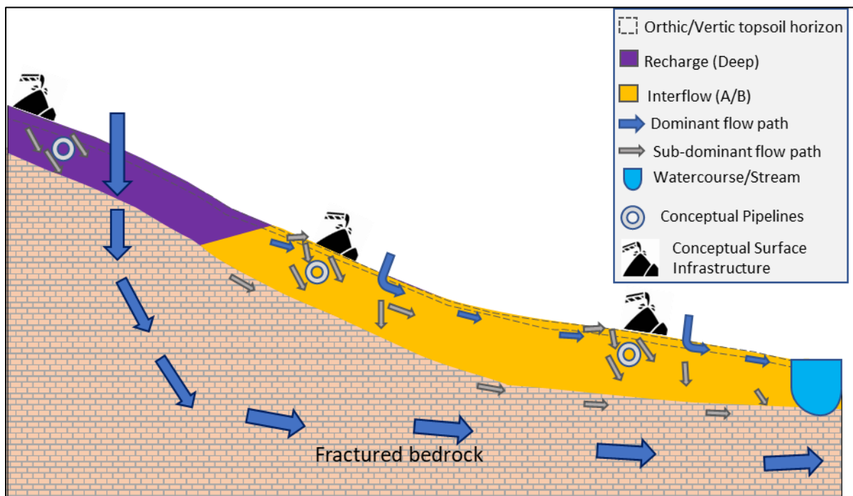
Figure 4-14 Hillslope hydrology one of five of the distinct hydropedological patterns after the construction of the Clover Alloys SA Plant Infrastructure Project and associated infrastructure
