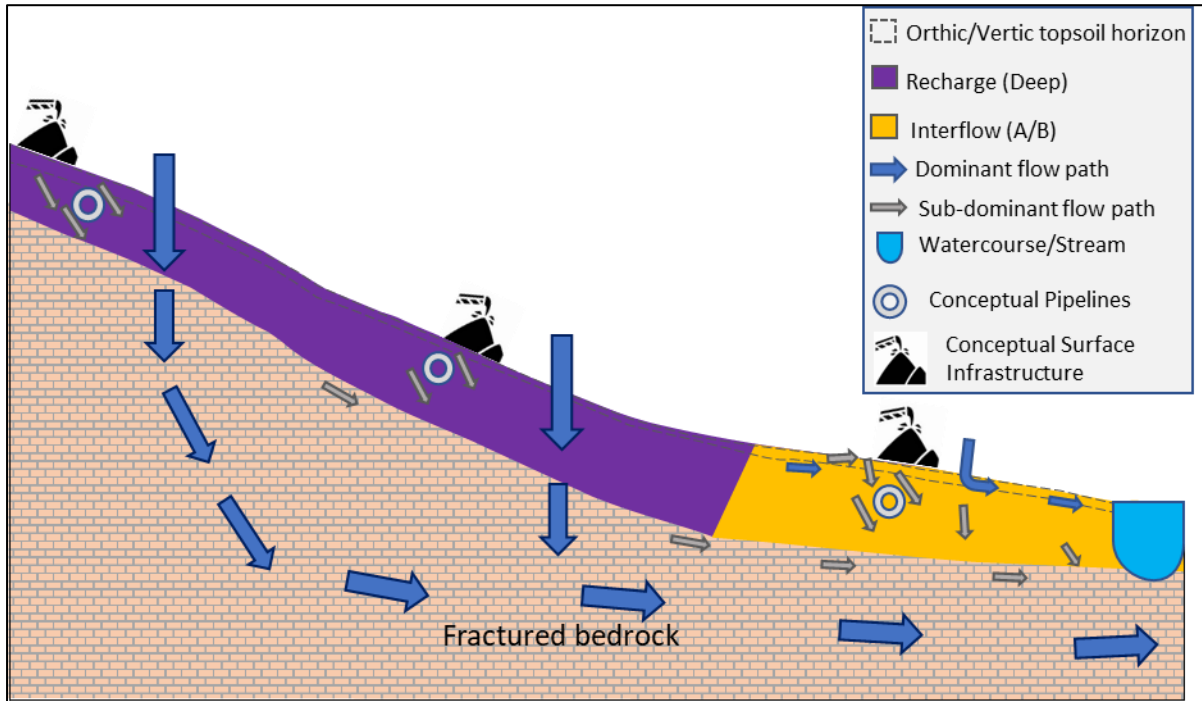
Figure 4-15 Hillslope hydrology two of five of the distinct hydropedological patterns after the construction of the Clover Alloys SA Plant Infrastructure Project and associated infrastructure
