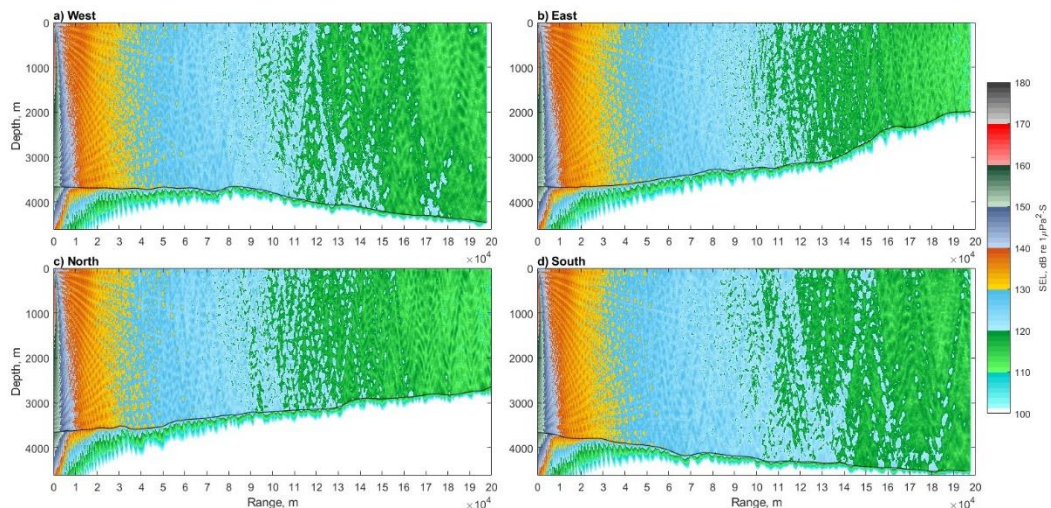
Figure 123: Modelled vertical contour images of the predicted SEL (unweighted) vs range and depth along the propagation path towards a) west b) east c) north and d) south direction from the source location L3. Black line shows the seabed depth.
